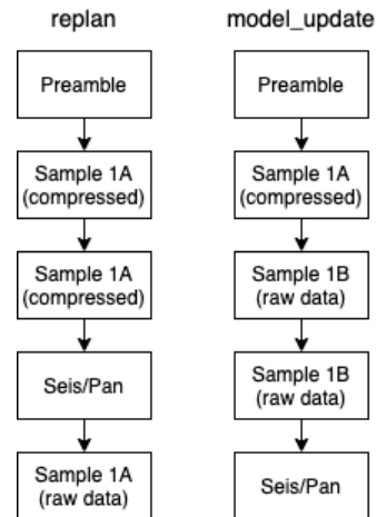
Figure 4. Sample high-level plans for the replan and model_update planning/execution strategies
