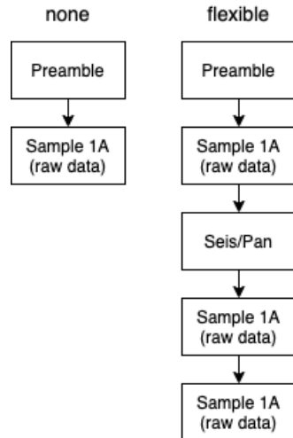
Figure 3. Sample high-level plans for the none and flexible planning/execution strategies.
