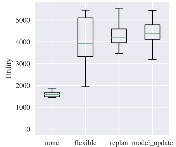
Figure 2. Average utility achieved by the four planning and execution strategies applied to simulated Europa Lander scenarios.
